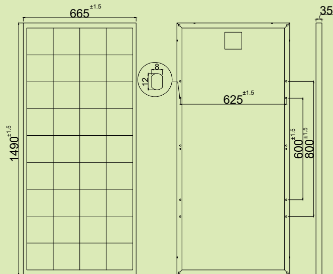
Frame Dimension
